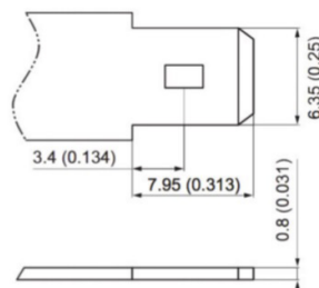
F2 Terminal Unit: mm (inches)
