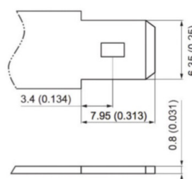
F2 Terminal Unit: mm (inches)
